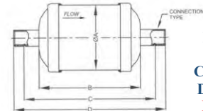
DCH BI-FLOW DRIER WITH ODF CONNECTION DIMENSIONS DRAWING 2
